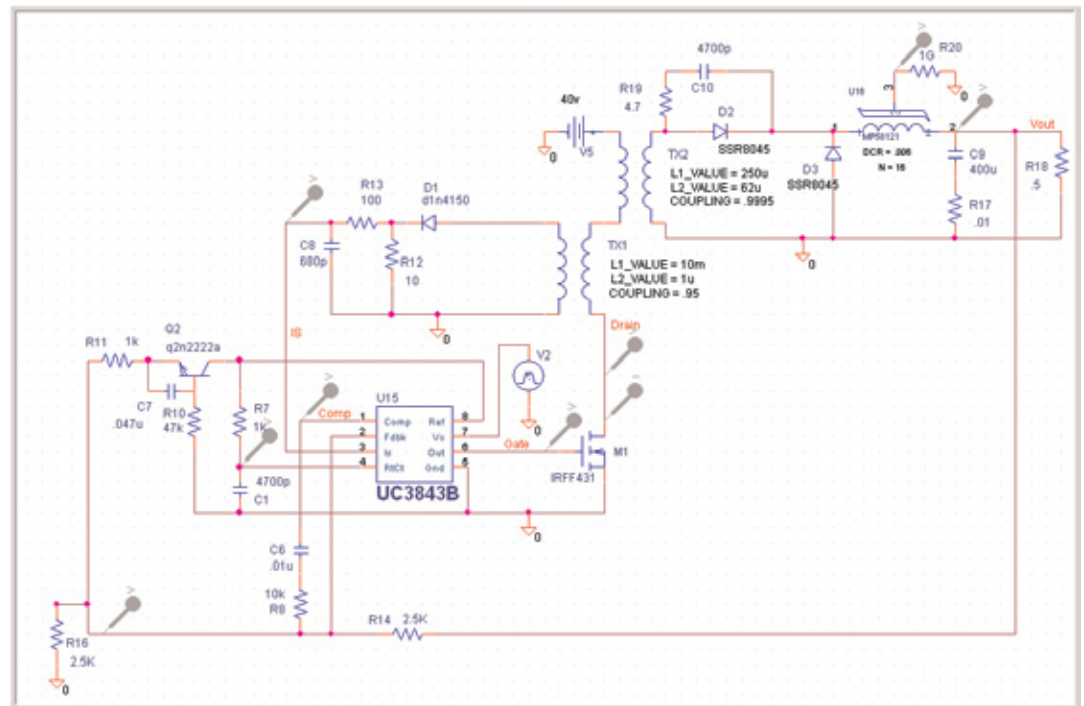
A 50W forward converter circuit using UC3843B PWM and Magnetics MPP58121 core models. The simulation explores the circuit operation as the transformer coupling is changed. The simulation can generate start up or steady state output depending on the settings
